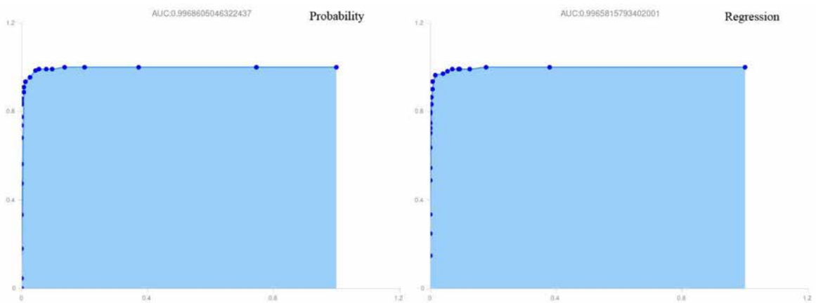
Fig. S2-C. Graphs of estimates of model accuracy by AUC-ROC for best probability and best regression of Random Forest for South-Eastern Kazakhstan.
