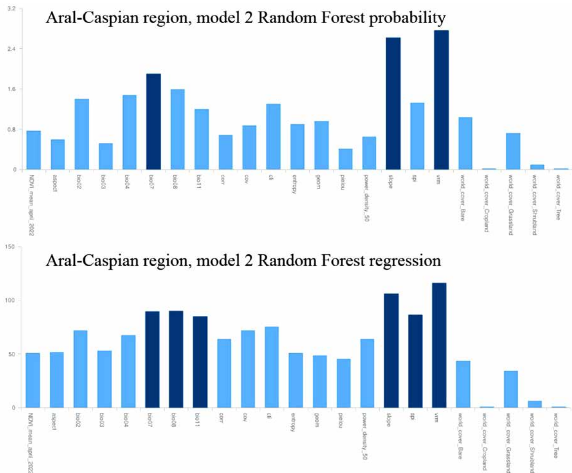
Fig. S1-A. Diagrams of important variables in Random Forest best models for Aral-Caspian region.
