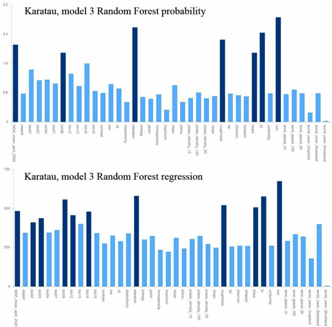
Fig. S1-B. Diagrams of important variables in Random Forest best models for Karatau region.
