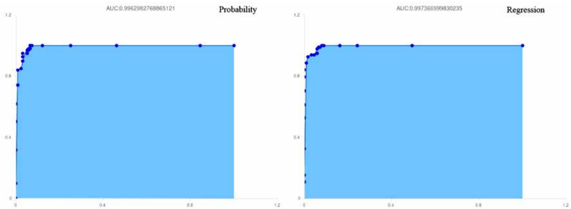
Fig. S2-A. Graphs of estimates of model accuracy by AUC-ROC for best probability and best regression of Random Forest for Aral-Caspian region.
