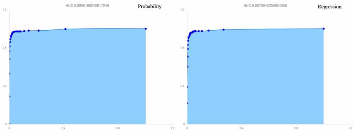
Fig. S2-B. Graphs of estimates of model accuracy by AUC-ROC for best probability and best regression of Random Forest for Karatau region.
